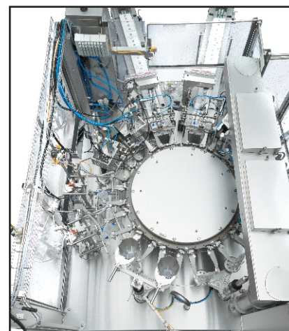
PSG LEE Duplex Pouch Fill-seal Machine
